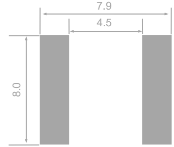
焊盘推荐尺寸 Recommended Pad Size (mm)
